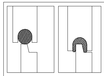
4. Base and cover sealed using the tongue and groove system.
